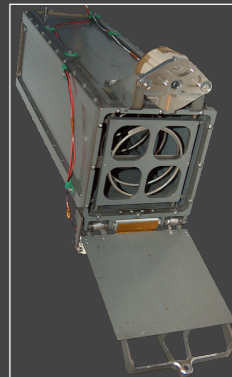
P-POD Deployer
