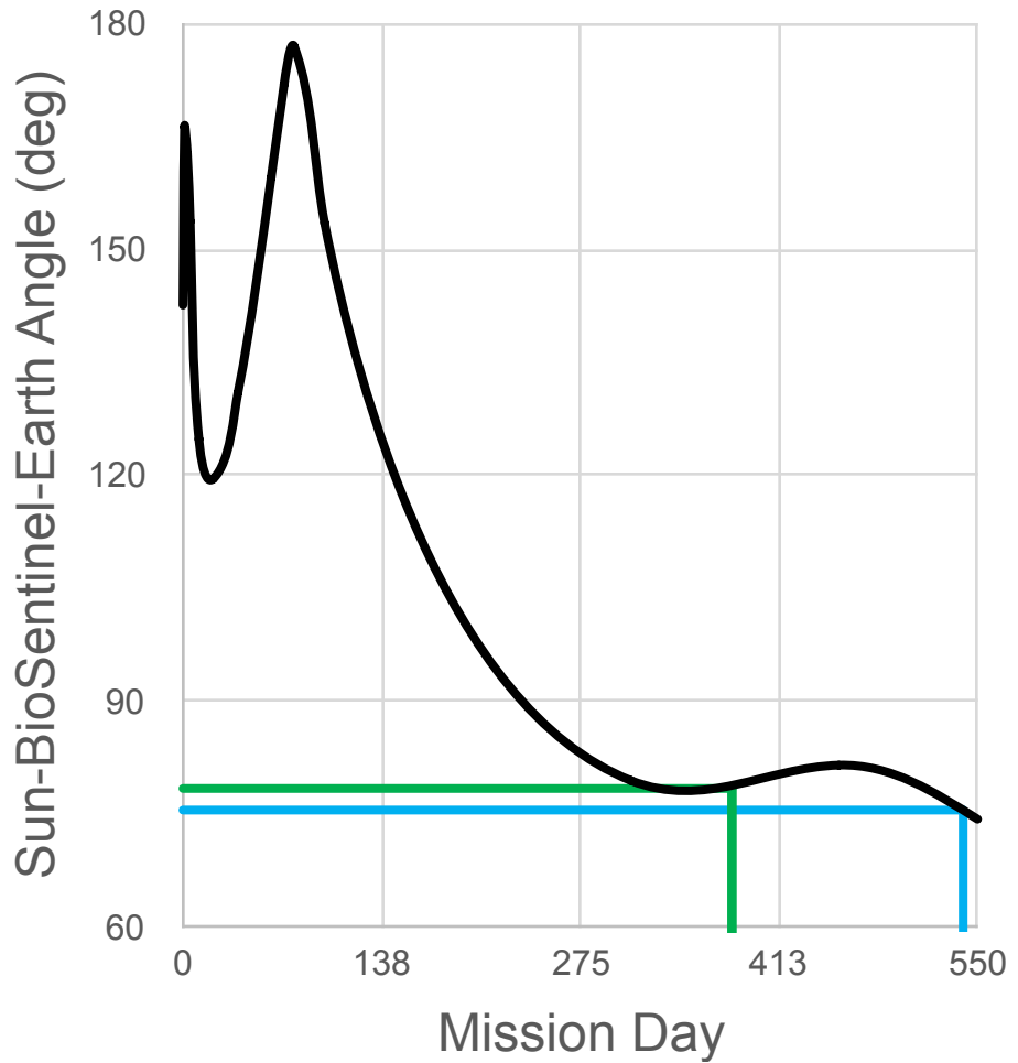
Sun-BioS-Earth Angle
