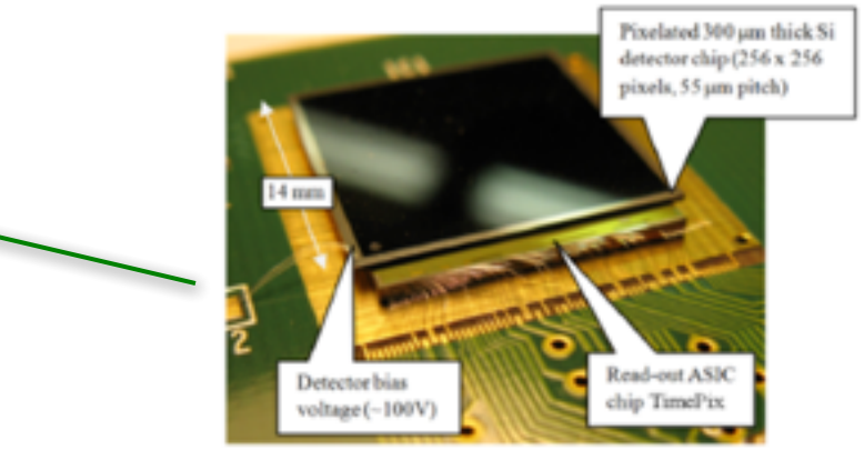
TimePIX Sensor
